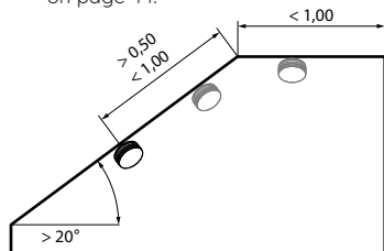
Fig. 14 Straight mounting surface less than 1 m long and 1 m wide
